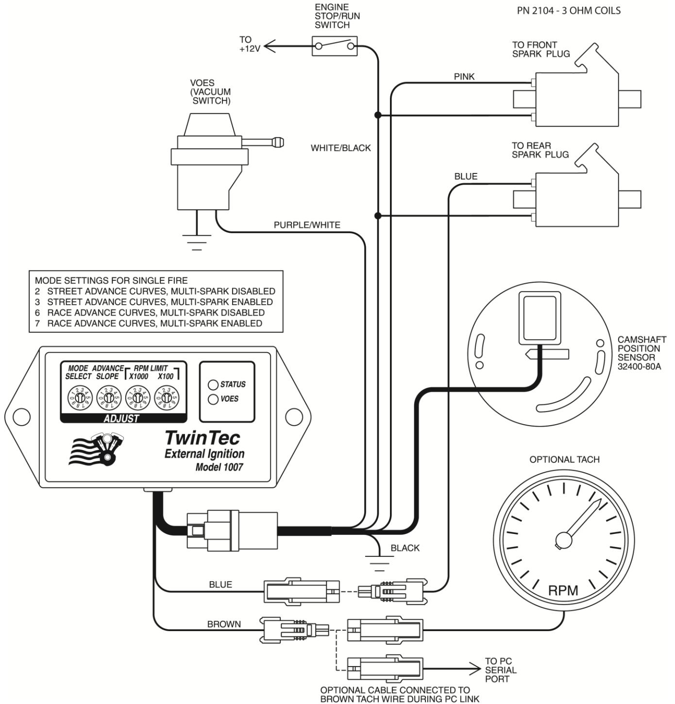
Figure 2 – Twin Tec Model 1006/1007 Wiring Diagram
